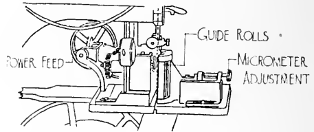
FIG. 185. RESAW ATTACHMENT FOR BAND-SAW.
